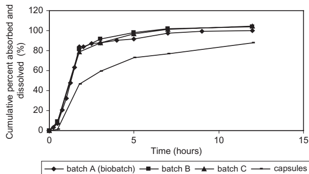
Figure 3. The results of dissolution tests for a 1000 mg dispersible tablets and 2 × 500 mg capsules and Wagner-Nelson plot of percentage of the dose absorbed versus time (batch A).
